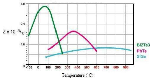
Figure 3: Performance of Thermoelectric Materials at various temperatures [4]
