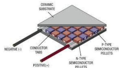
Figure 1: Seebeck effect [11]
