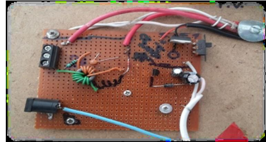
Figure 7: Joule Thief Converter (Booster circuit) used in present study
