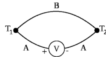
Figure 1: Seebeck effect [11]
