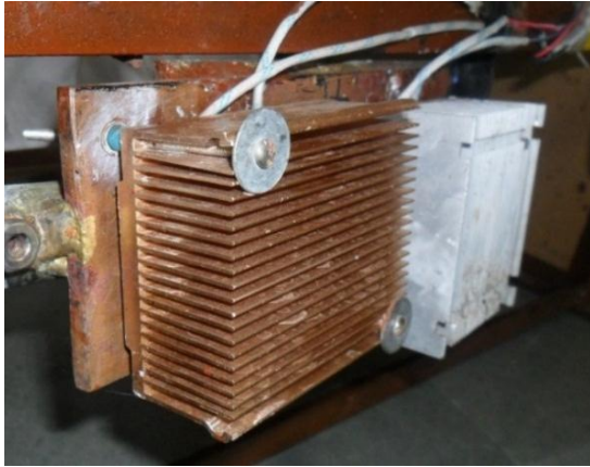
Figure 9: TEG Setup fabricated for present study
