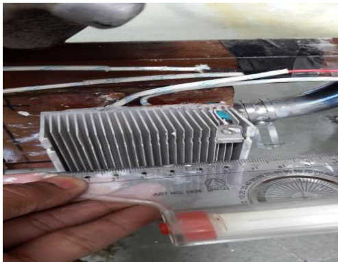
Figure 6. Aluminum heat sink fabricated for the present study
