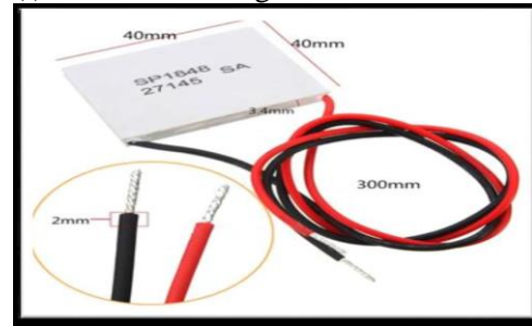
Figure 4. Thermoelectric generator
