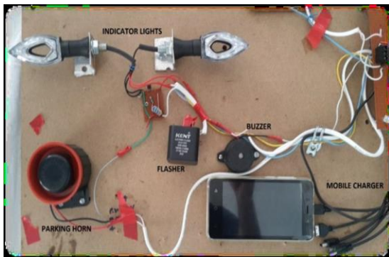
Figure 8: Load attached across TEG in the present study
