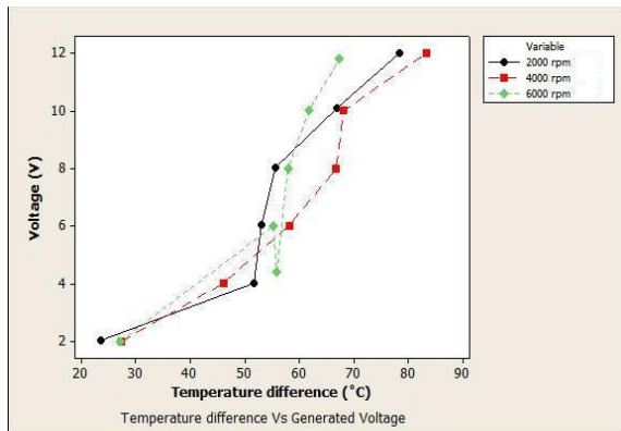
Figure 12: Shows that temperature difference is directly proportional to voltage
