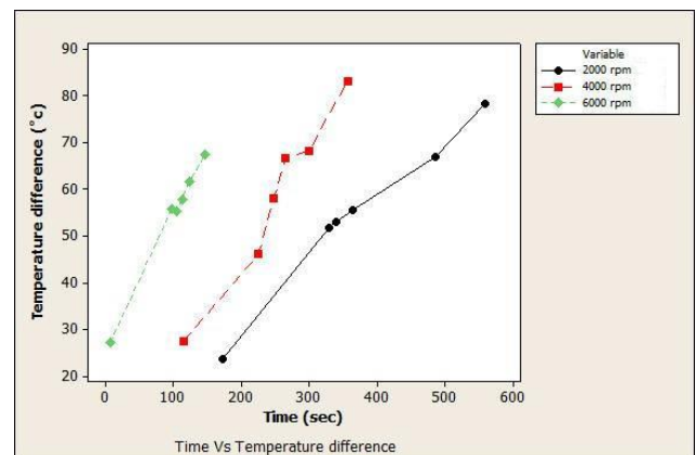
Figure 11: Shows that time is directly proportional to temperature difference.
